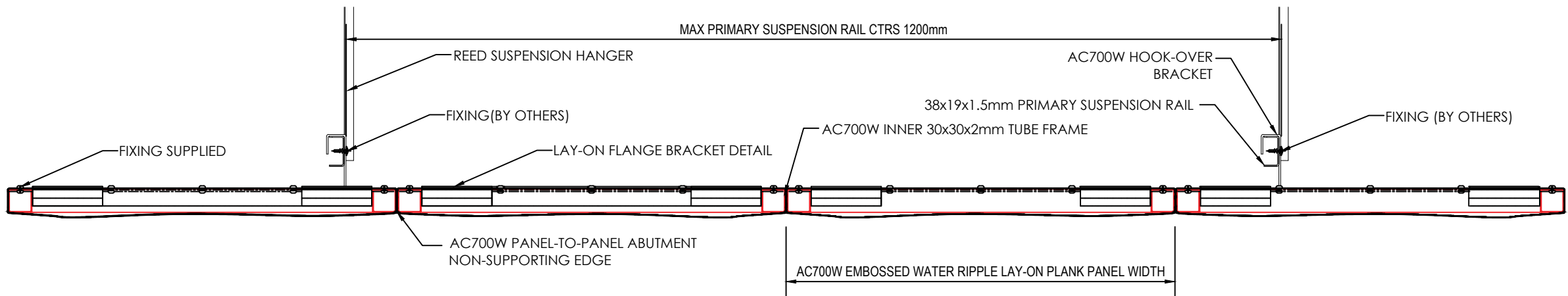
03 AC700W - CROSS SECTION (NON-SUPPORTING DETAIL) SCALE AS PER MODEL
