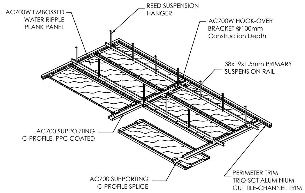
01 AC700W - ISOMETRIC VIEW NTS
