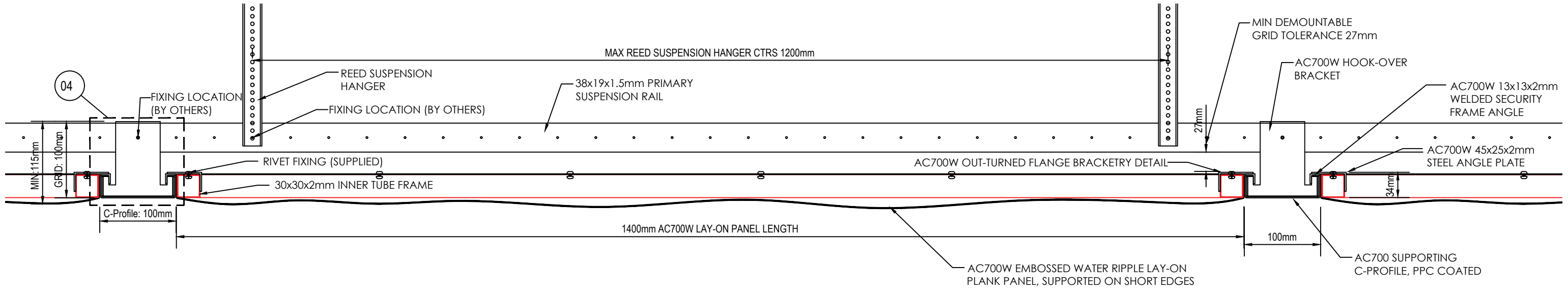
02 AC700W - LONG SECTION (SUPPORTING DETAIL) SCALE 1:1
