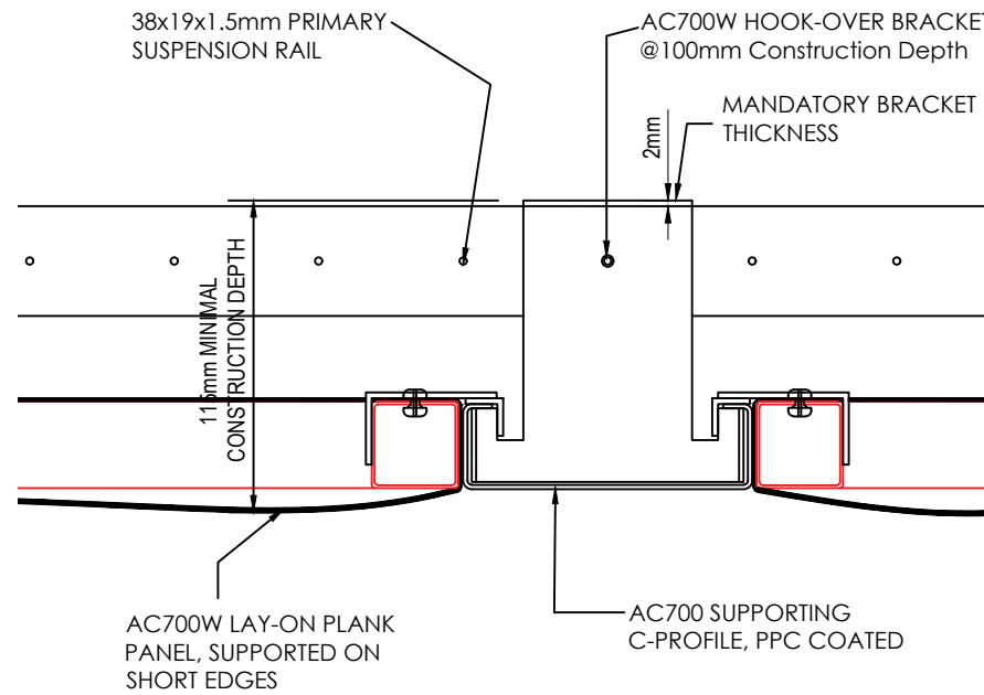
04 AC700W - ENLARGED DETAIL SCALE 1:1
