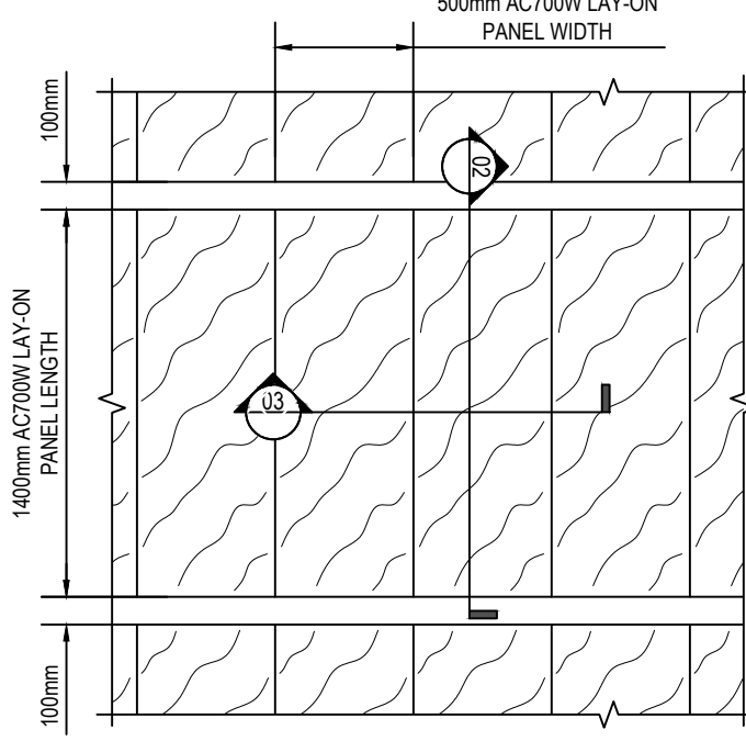
01 AC700W - RCP VIEW SCALE 1:30
