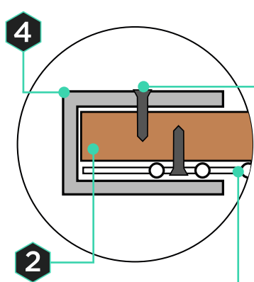
Plan View: Panel configuration detail
