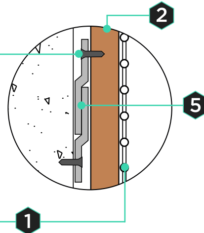
Side View: Mounting detail
